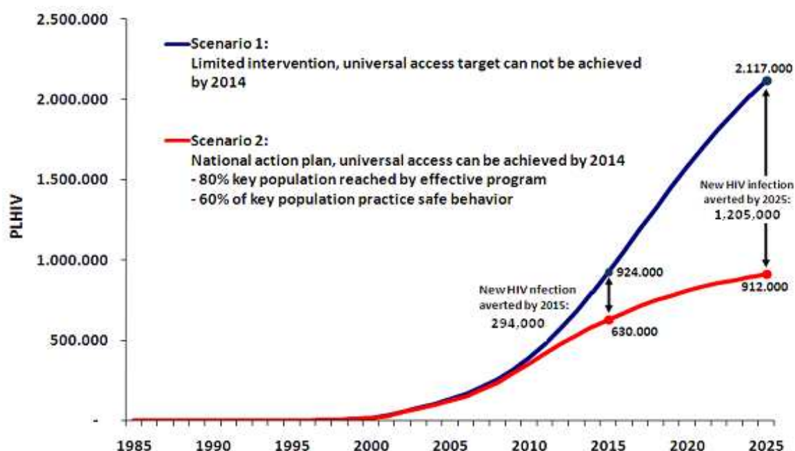
Figure 2. Projection of UA Achievements with Different Scenarios
